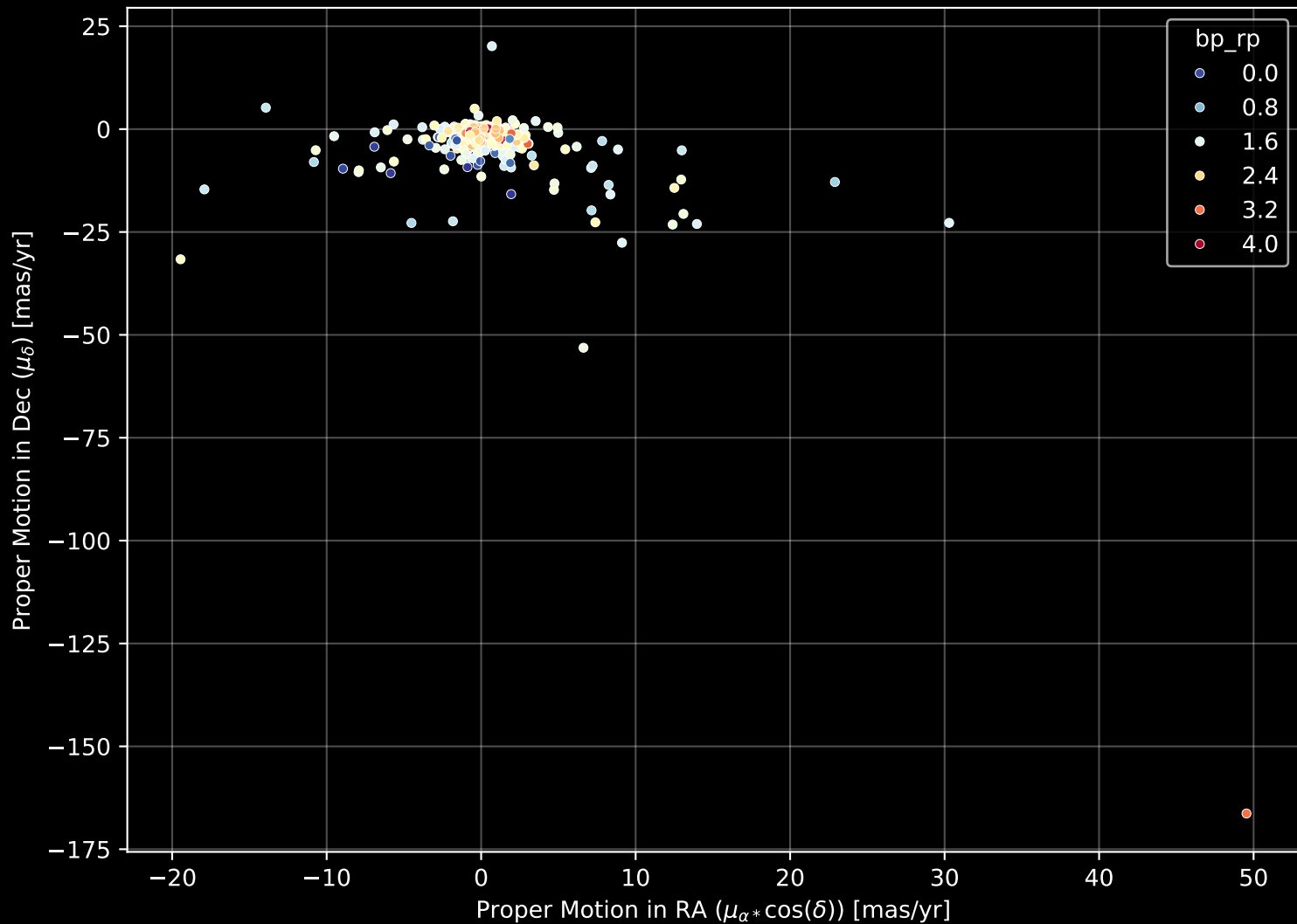
APOGEE DR17 Field: [195+00] Proper Motion Diagram (n= 495)
