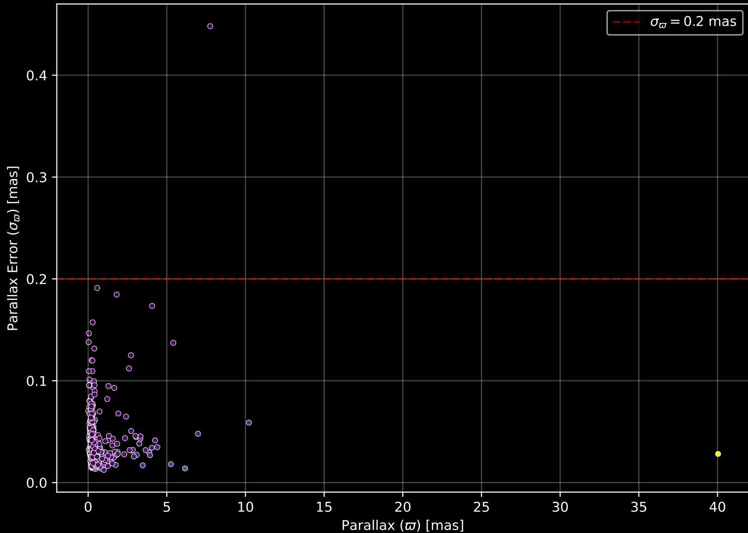
APOGEE DR17 Field: [195+00] Parallax Quality (n= 495)
