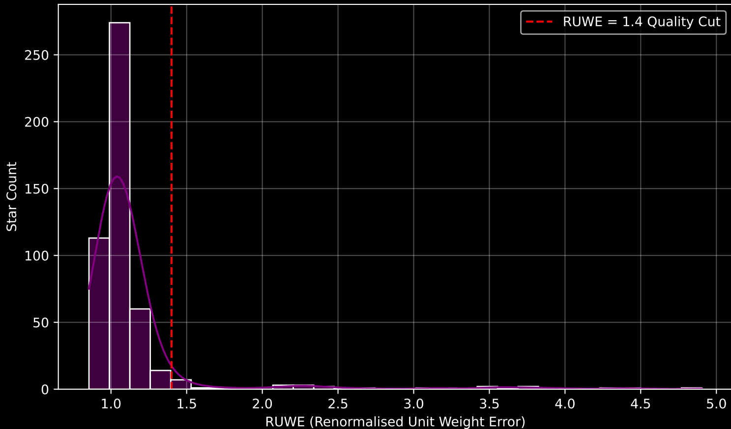
GAPOGEE DR17 Field [195+00] RUWE Distribution (n= 492)
