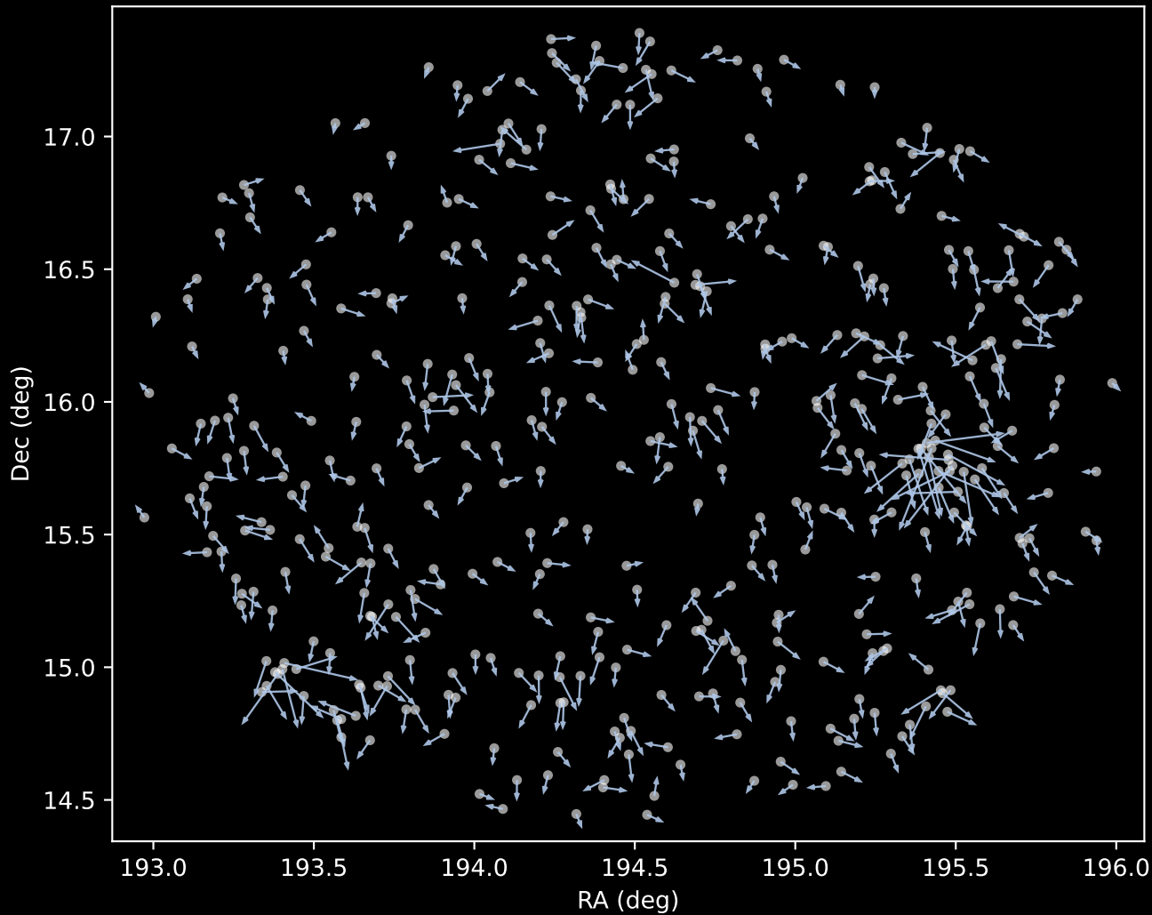
APOGEE DR17 Cluster 1 Proper Motion Vectors (n=459)
