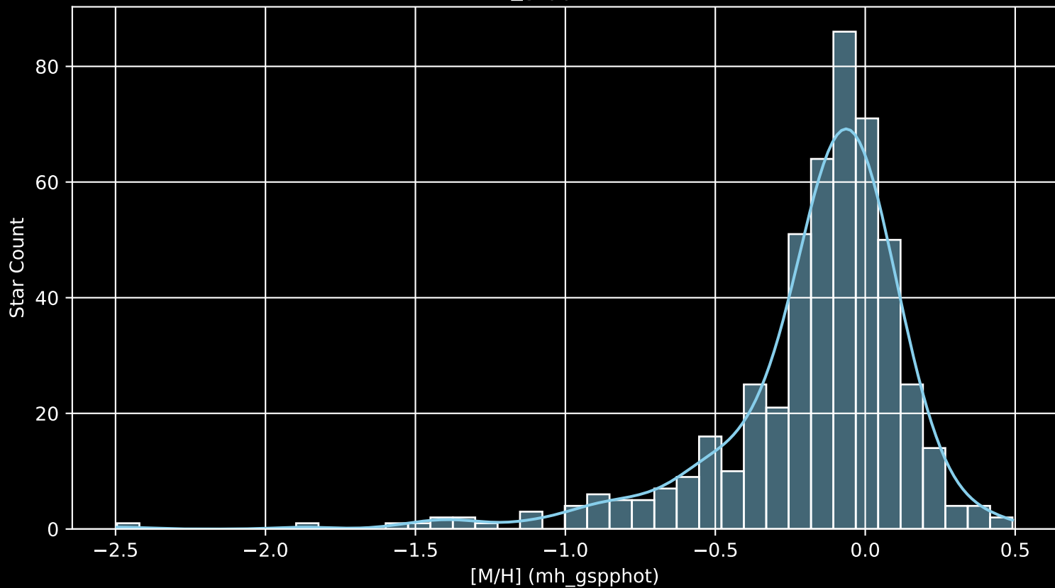
APOGEE DR17 Field: [195+00 [M/H] (mh_gspphot) (n= 491)
