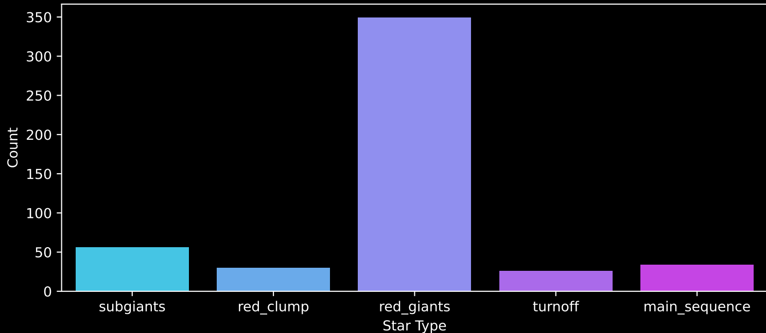
APOGEE DR17 Field: [195+00] Count plot of Star Type
